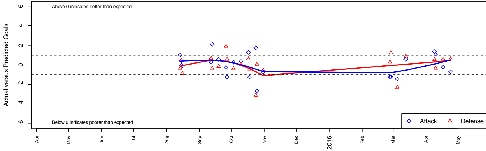
Capital FC Timbers White G01 Dots are actual minus expected GF (blue circles) and GA (red triangles). Blue line is smoothed change in attack strength. Red is smoothed change in defense strength.
